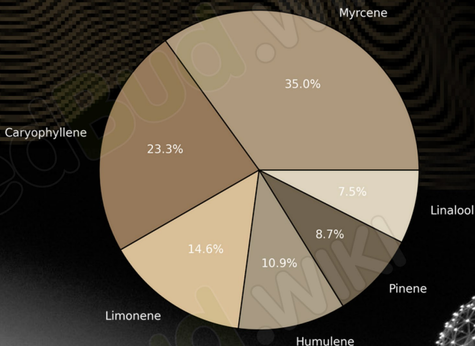
Interstellar Terpene Profile
